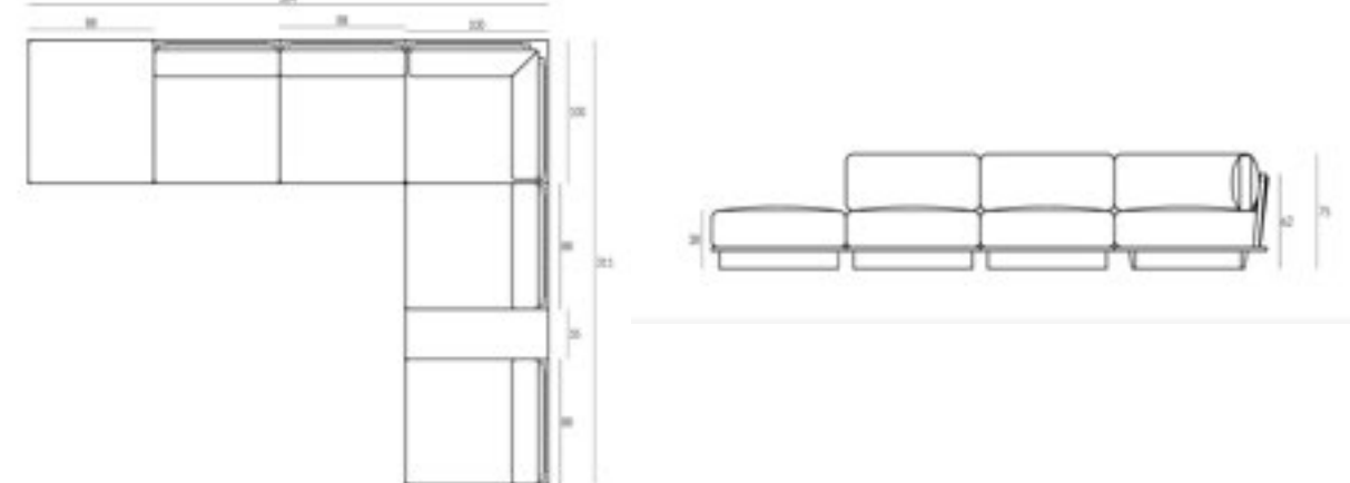
OTTOMAN / 2 X CENTRE SECTIONS / CORNER / CENTRE SECTION / SIDE TABLE / OTTOMAN
